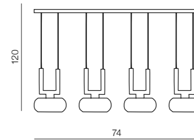
Rubic 4 A AZ0494 G9 4x 40W metal/chrome/acryl
