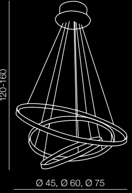
LED Wheel 3 Big AZ1431 (chrome) LED 70.5W 4600 lm chrome/metal
