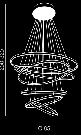
LED Wheel 6 AZ1280 (chrome) LED 135W 8800 lm chrome/metal
