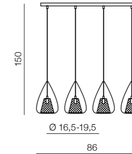
Gordon 4 Line AZ2170 G9 4x MAX 33W metal/glass
