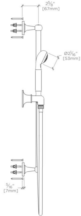
SIDE VIEW
