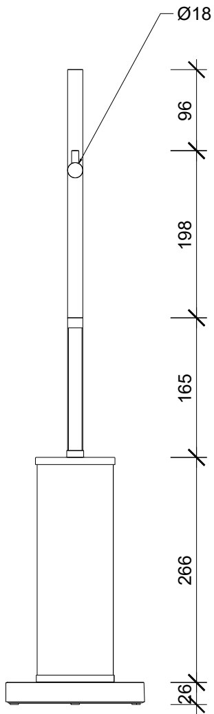
Frontansicht front view
