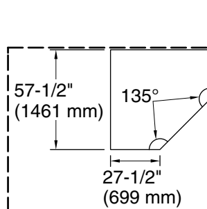
Drop-In Rim Style Cut-Out Detail
