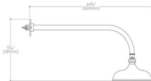
SIDE VIEW SCALE: 1\frac{1}{2}''=1'-0''
