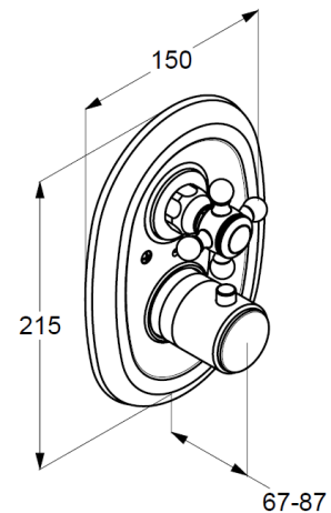
Dimensional drawing
