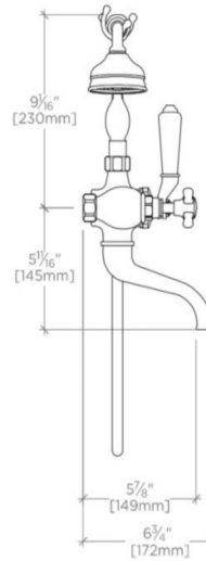
SIDE VIEW SCALE: 1 1/2"=1'-0"
