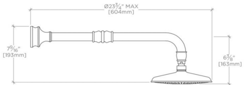
SIDE VIEW SCALE: 1 1/2"=1'-0"
