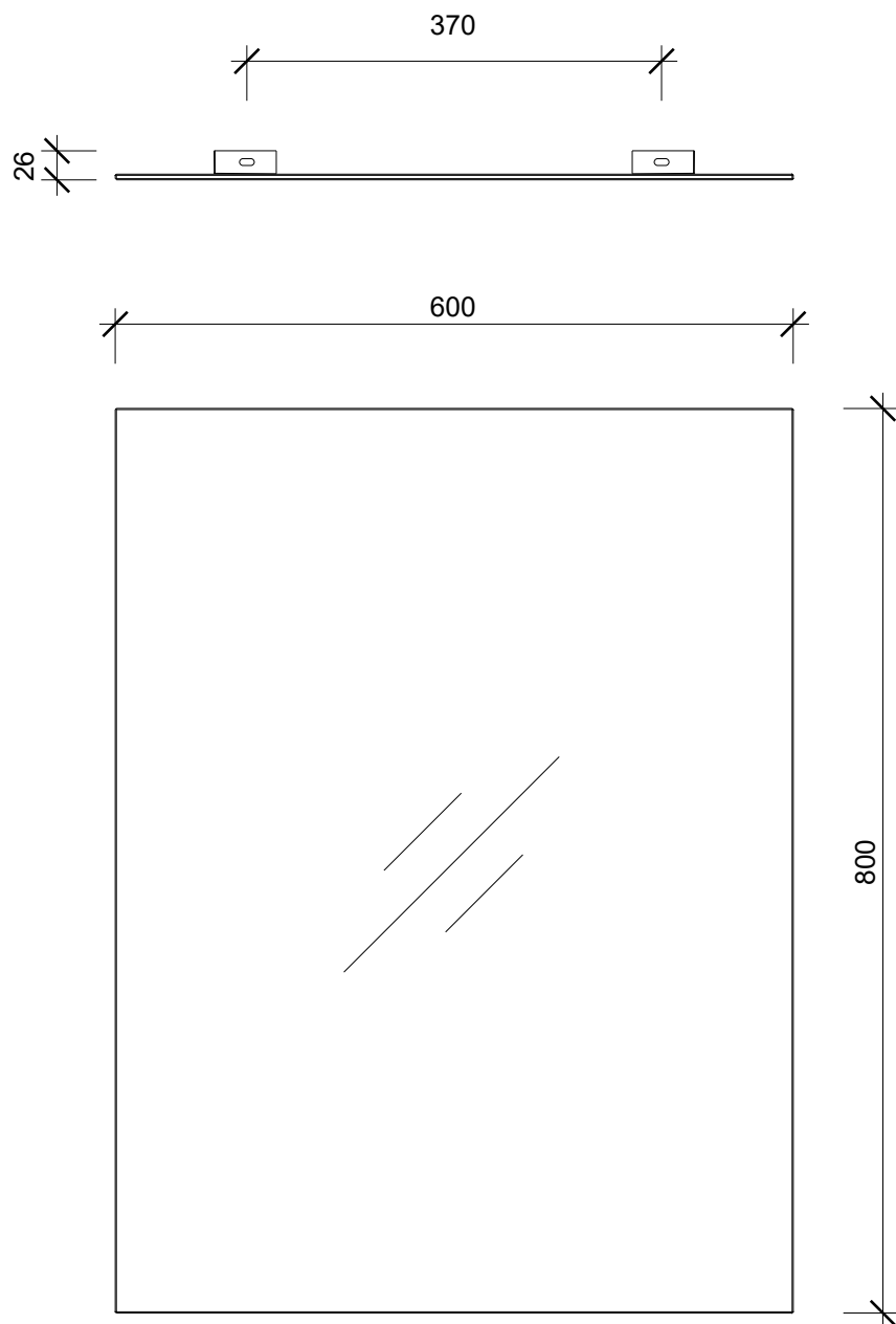
Frontansicht front view
