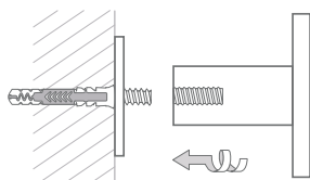
Montage HA3-R40S55-B:
