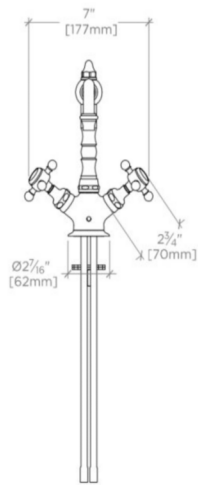
FRONT VIEW SCALE: 1 1/2"=1'-0"
