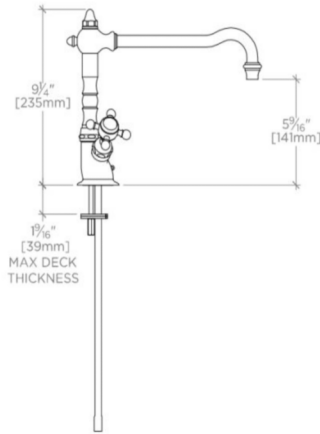
SIDE VIEW SCALE: 1 1/2"=1'-0"
