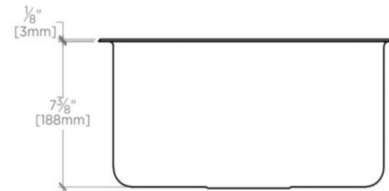
SIDE VIEW SCALE: \frac{1}{2}"=1'-0"
