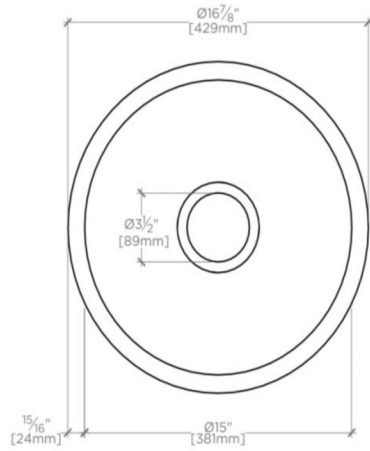
TOP VIEW SCALE: \frac{1}{2}"=1'-0"
