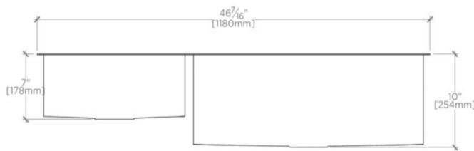
FRONT VIEW SCALE: 1"=1'-0"
