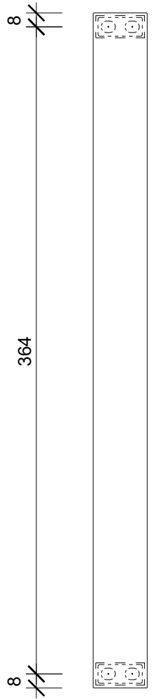
Frontansicht front view
