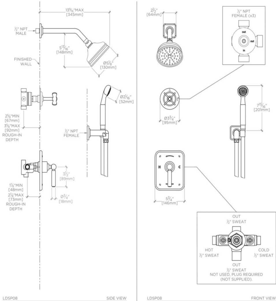
LDSP08 SIDE VIEW THIS DRAWING IS NOT INTENDED FOR USE AS A PIPING SCHEMATIC
