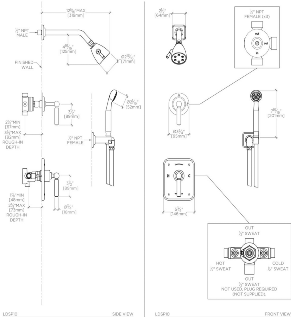
LDSP10 SIDE VIEW THIS DRAWING IS NOT INTENDED FOR USE AS A PIPING SCHEMATIC
