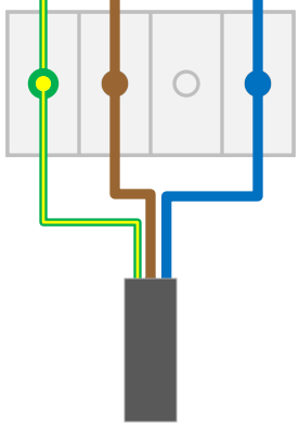
230v POWER IN
