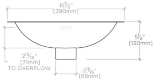
FRONT VIEW SCALE: 1/2"=1'-0"
