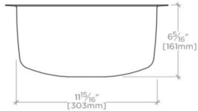
SIDE VIEW SCALE: 1/2"=1'-0"
