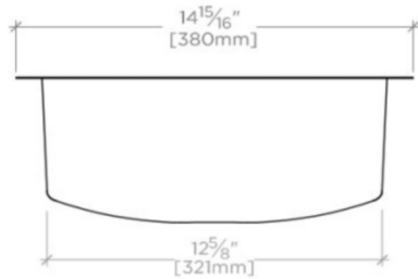
FRONT VIEW SCALE: 1/2"=1'-0"
