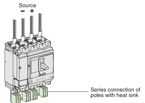
ComPact NSX DC - safety and flexibility.
