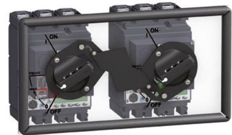
Interlocking of two devices with rotary handles.
