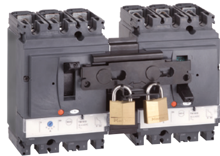
Interlocking of two or three toggle-controlled devices.
