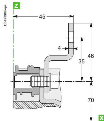
NSX100 to 250 DC
