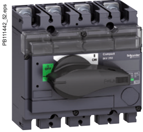
ComPact INV250 switch-disconnector.
