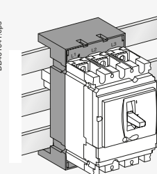
Mounting on busbars with an adapter.
