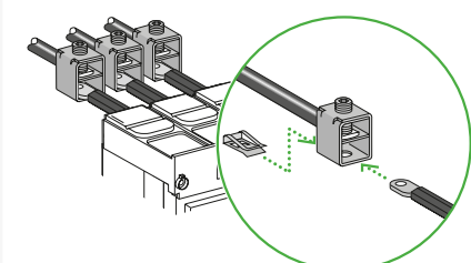
Connection of bare cables to NSX100 to 250 DC by clips.
