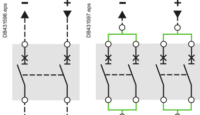
Selection 1. Selection 2: ComPact NSX160 DC 4P 2 x 2P parallel mounted in series.
