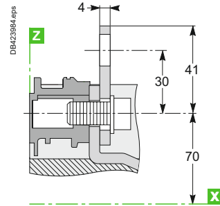
NSX400/630 DC
