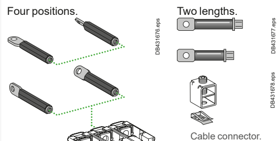
Cable connector.
