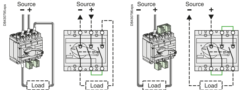
One type of connection per frame size, two catalog numbers for all series connections.
