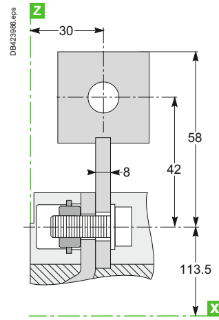
NSX400/630 DC
