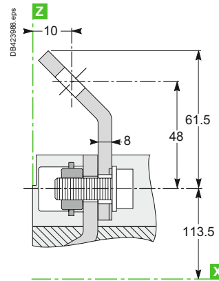
NSX400/630 DC
