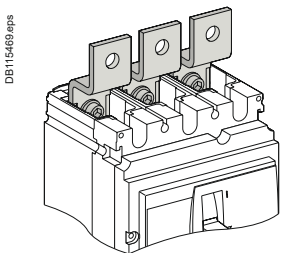
Double-L terminal extensions
