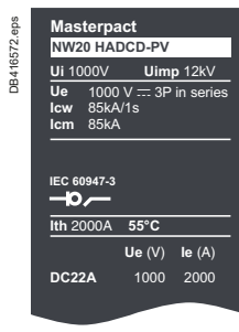
NW20 HADCD-PV rating plate.
