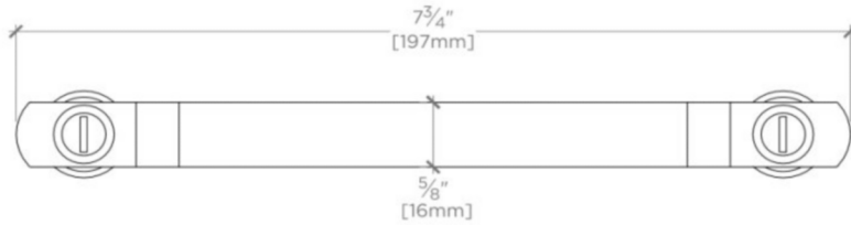
FRONT VIEW
