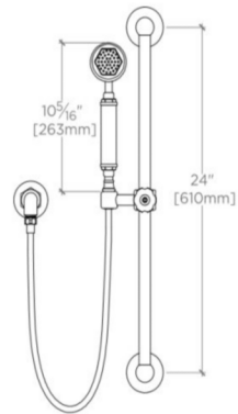
FRONT VIEW SCALE: 1"=1'-0"
