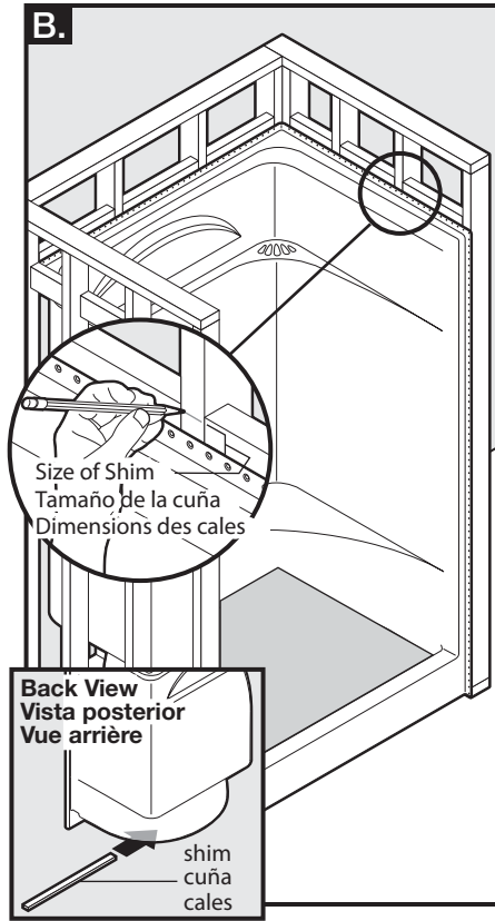
B. Check level left to right and front to back.
