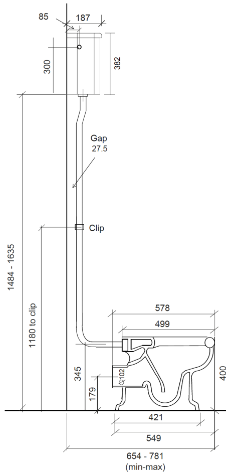
Side view with p-trap pan
