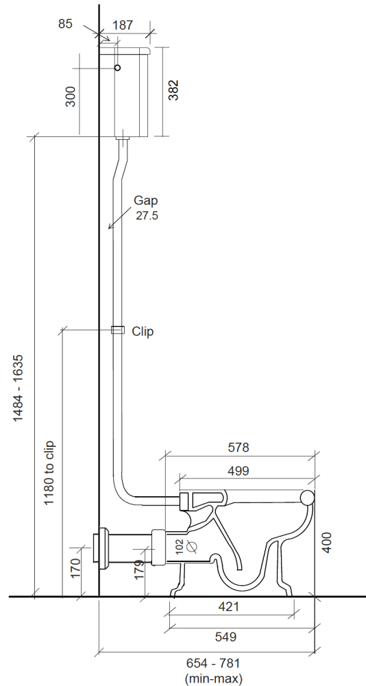
Side view with optional vertical pan connector
