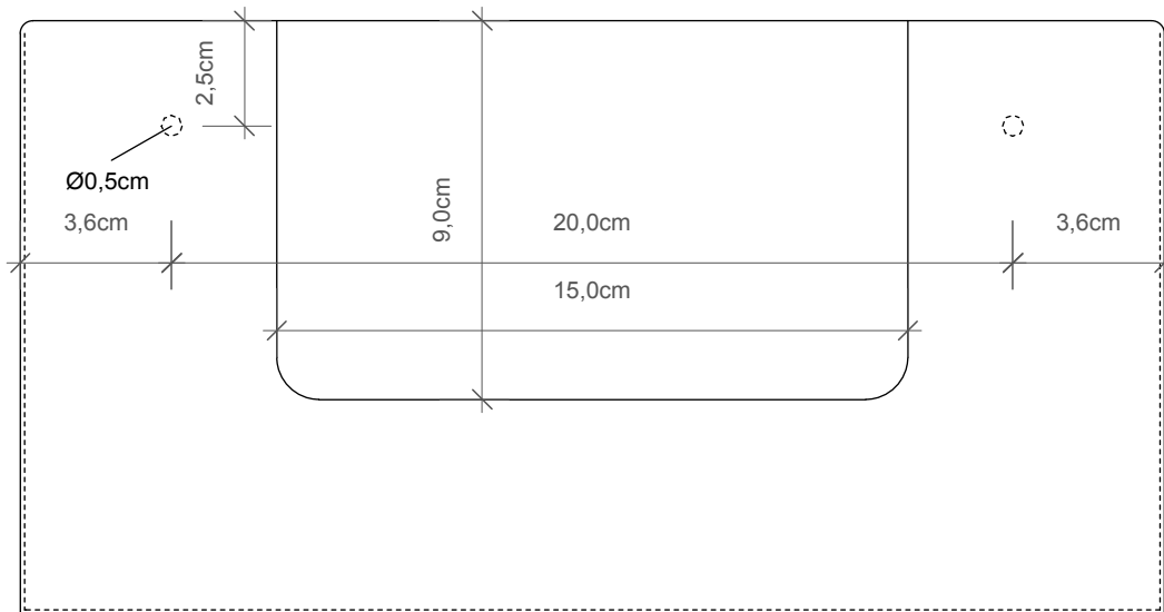
Frontansicht Front view
