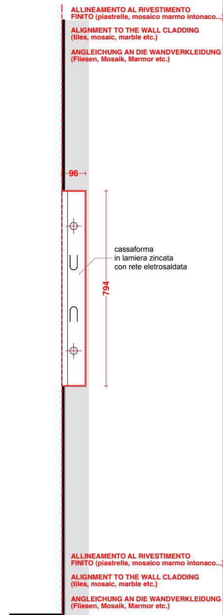
cassaforma formwork
