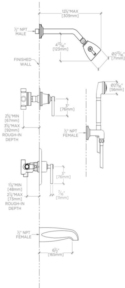
TRSP16 SIDE VIEW
