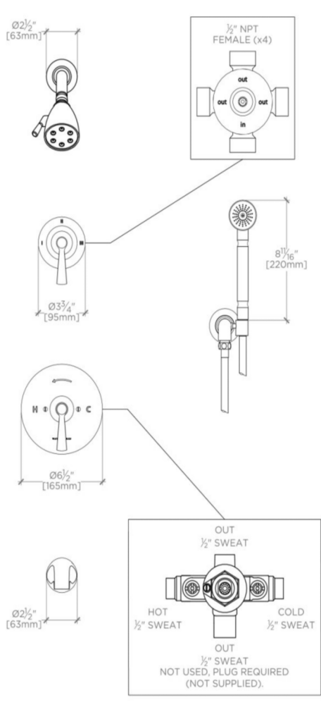
TRSP16 FRONT VIEW
