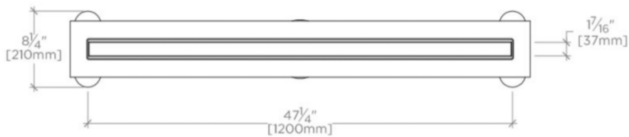
TOP VIEW
