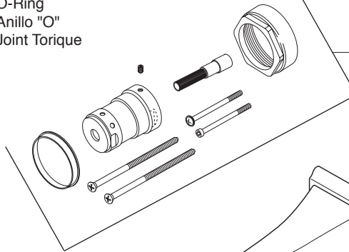
RP75136 Extension Kit Extension para la kit Rallonge de kit
