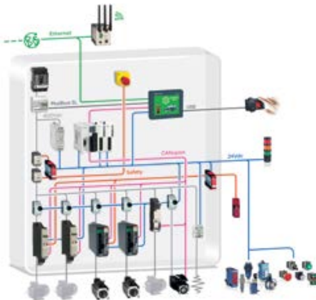
Example of TVDA Compact / CANopen / HMI Controller SCU embedding Zelio solid-state relays e.g. for heating unit control.
