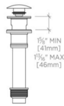
SIDE VIEW SCALE: 1 1/2"=1'-0"
