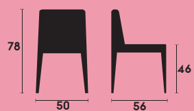
Ref. 630 Silla. / Chair.
