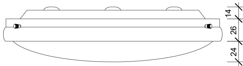
Frontansicht front view
