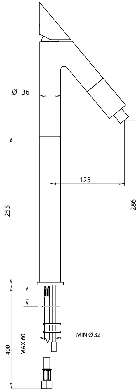
Basin mixer with 250 mms extension and clic-clac waste
