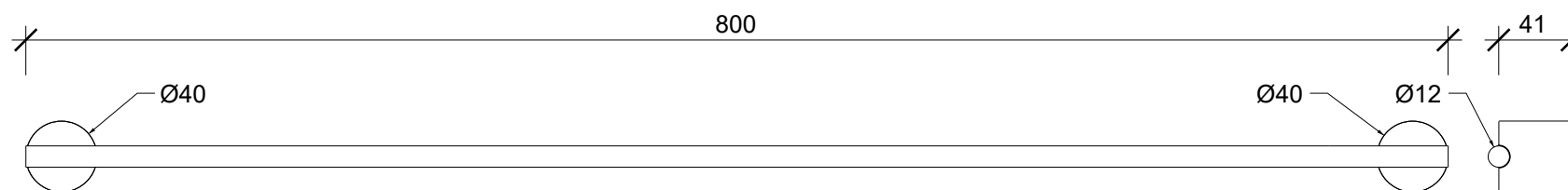
Frontansicht front view
