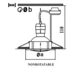
NONROTATABLE
