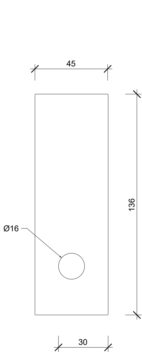
Frontansicht front view
