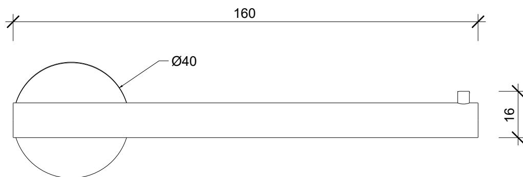
Frontansicht front view
