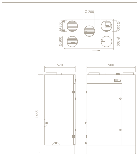
Dimensioni (lxhxp): 900x1465x570 mm
