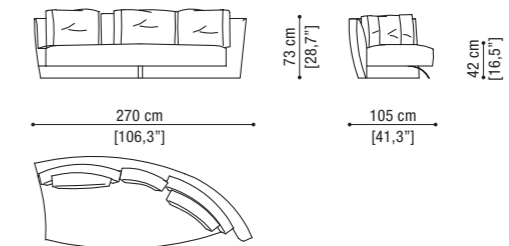
Terminal unit left/right 3,5 seater
