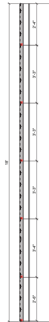
VERTICAL SECTION 2 Scale 1:10
