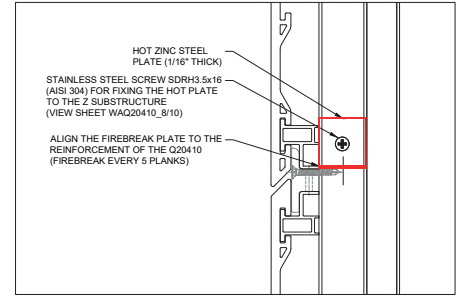
VERTICAL SECTION 2 Scale 1:10
